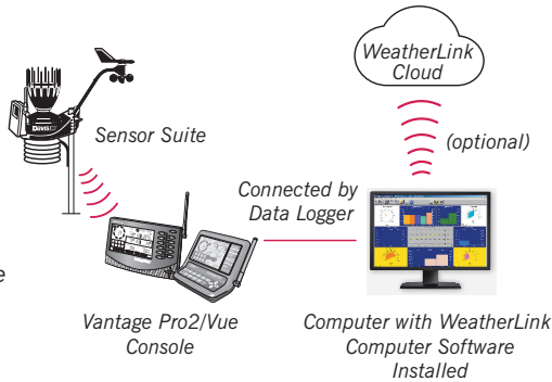
Data loggers compatible with Vantage Vue and Vantage Pro2 consoles.
